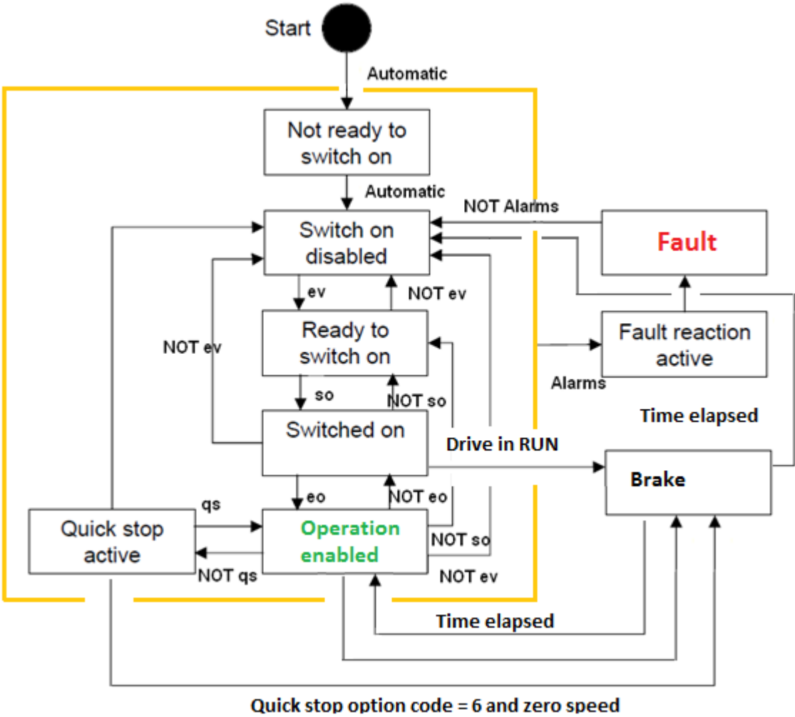
Fig. 1- Drive State Machine
