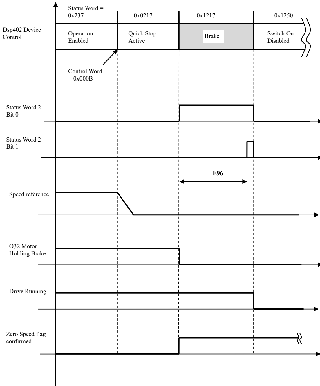
Fig. 21-Quick stop
