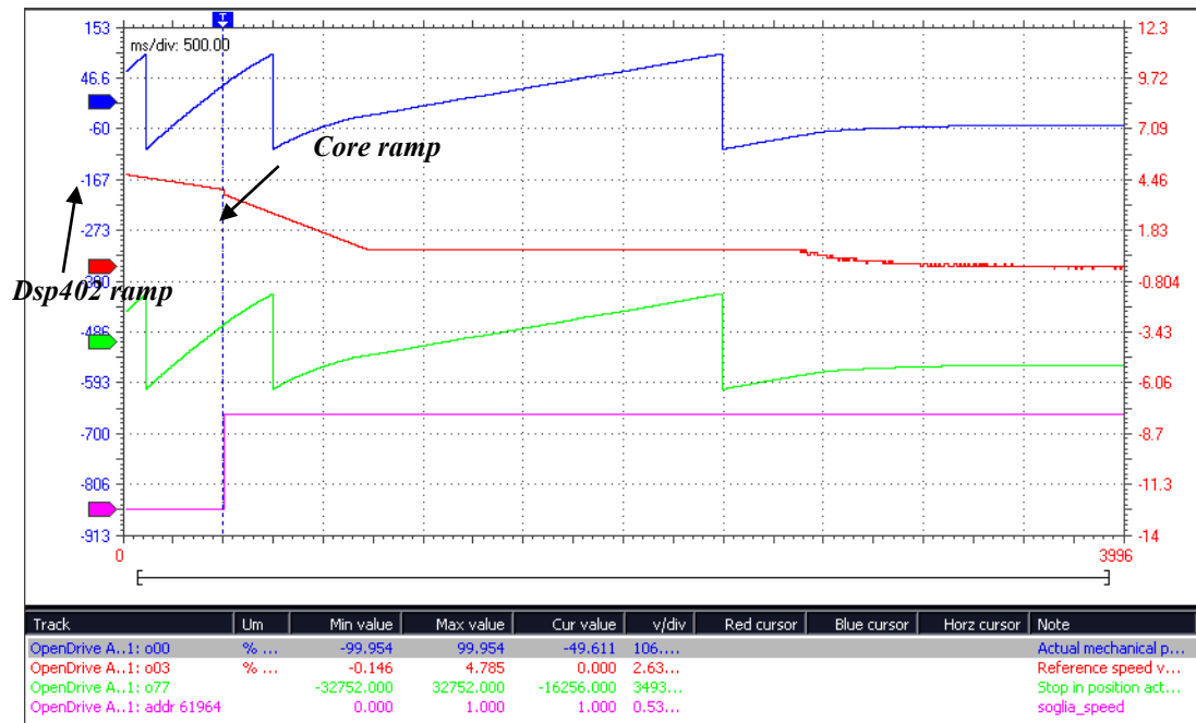
Fig. 16-Application's ramps
